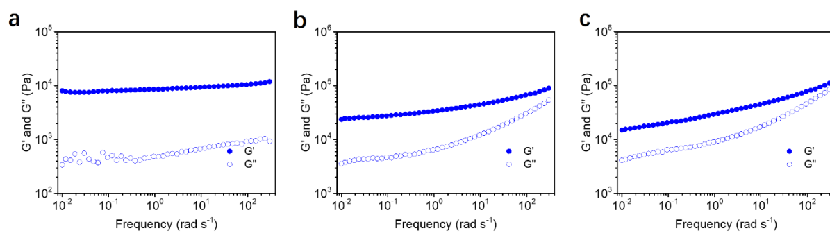
Figure S1. The storage modulus G' and the loss modulus G'' as a function of angular frequency of poly(ATAC-co-PEA) hydrogels with different PEA molar fraction f . (a) f = 0.7 , (b) f = 0.8 , (c) f = 0.85 .
