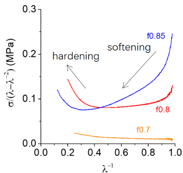
Figure S3. Mooney–Rivlin curves of poly(ATAC-co-PEA) hydrogels with different PEA fraction f . \sigma is stress and \lambda is the extension ratio, which is related to the strain \varepsilon as \lambda = \varepsilon + 1 .
