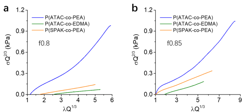
Figure S9. Normalized tensile stress-extension ratio curves of hydrogels with different monomer pairs in water. (a) f=0.8 . (b) f=0.85 . \sigma is stress of hydrogels. \lambda is the extension ratio, which is related to the strain \varepsilon as \lambda = \varepsilon + 1 . Q is the volume swelling ratio of hydrogels in relative to their as-prepared states.
