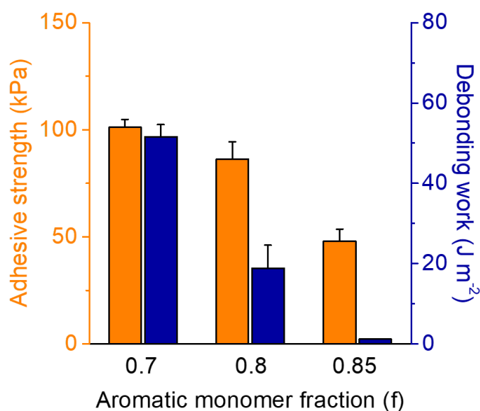
Figure S8. Adhesion values of poly(ATAC-co-PEA) hydrogels with different PEA fraction f in 0.7 M NaCl solution. All samples were reached equilibrium in 0.7 M NaCl. Error bars indicate standard deviation ( N = 5 ). All the tack tests were performed on a glass substrate. The pressures of tack test were equivalent to 100%E, 50%E, 30%E of f = 0.7 , f = 0.8 , and f = 0.85 gels, respectively, where E is the elastic modulus of the corresponding hydrogels.
