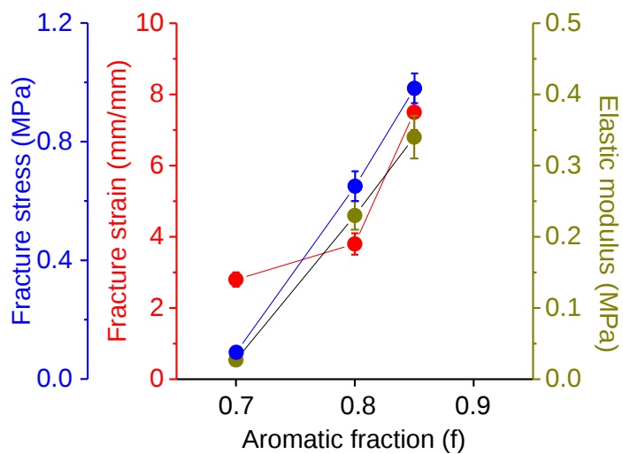
Figure S2. The fracture stress, fracture strain, and elastic modulus of poly(ATAC-co-PEA) hydrogels with different f obtained from stress–strain curves in Figure 2d of the main text.
