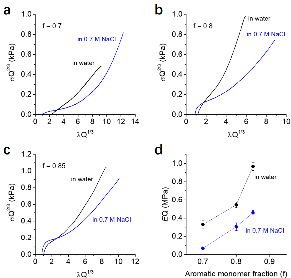
Figure S7. (a-c) Normalized tensile stress-strain curves of poly(ATAC-co-PEA) hydrogels in water and in 0.7 M NaCl solution. (a) f = 0.7 . (b) f = 0.8 . (c) f = 0.85 . \sigma is stress of hydrogels. \lambda is the extension ratio, which is related to the strain \varepsilon as \lambda = \varepsilon + 1 . Q is the volume swelling ratio of hydrogels in relative to their as-prepared state. (d) Normalized elastic modulus of hydrogels in water and in 0.7 M NaCl solution.
