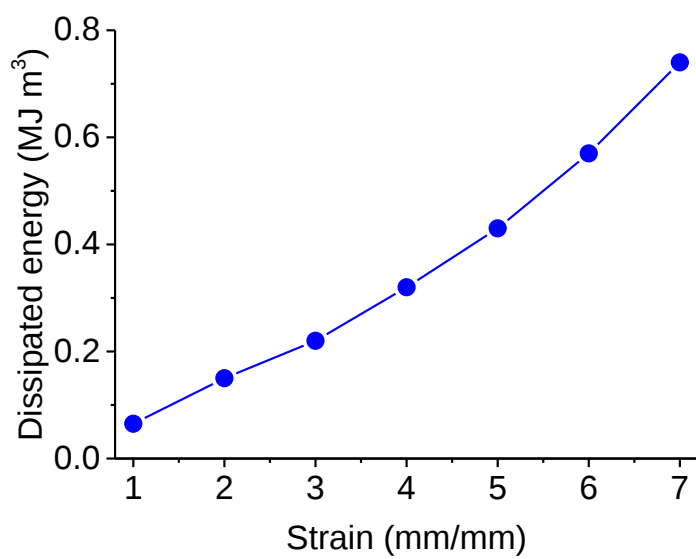
Figure S4. The dissipated energy of poly(ATAC-co-PEA) hydrogel ( f = 0.85 ) under different strain.
