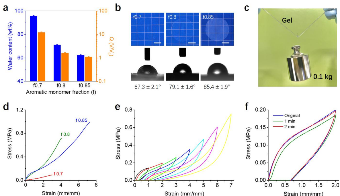
Figure 2. Mechanical properties of poly(ATAC-co-PEA) hydrogels with different aromatic monomer fractions ( f ). a) Water content and swelling ratio of hydrogels. b) Digital photos and contact angle of hydrogels to water. c) A digital photo showing that a string of tough hydrogel ( f = 0.85 ) can hold a load. d) Tensile stress-strain curves of hydrogels with different f values. e) Representative cyclic tensile loading-unloading curves with a gradual strain increase for the f = 0.85 hydrogel. f) Hysteresis and self-recovery of the f = 0.85 hydrogel measured by cyclic tensile tests. The initial strain rate of tensile tests was 0.14 \text{ s}^{-1} . The numbers in (b) and (d) are the f values.
