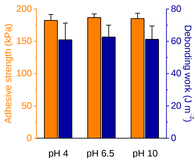
Figure S5. Adhesion values of poly(ATAC-co-PEA) hydrogels ( f = 0.85 ) in water of different pH values. Error bars indicate standard deviation ( N = 5 ). The tack tests were performed at a normal pressure equivalent to the elastic modulus E of the gels. All the tests were performed on a glass substrate. The acidic and basic solutions were prepared by dissolving HCl and NaOH in water, respectively. The ionic strength of pH 4 and pH 10 solutions was \sim 10^{-4} M. The swelling ratio and mechanical properties of the hydrogels in pH 4 and pH 10 solutions were the same as that in water (pH 6.5).
